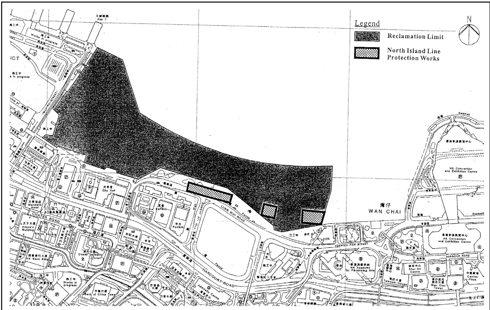
Figure 4: North Island Line Protection Works – Layout Plan
